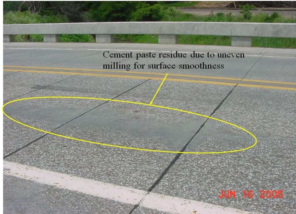
Figure 19. Cement paste cover was milled off leaving steel fibers exposed
