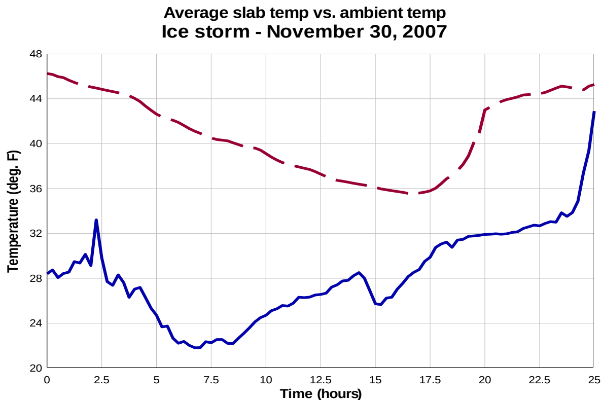
Figure 27. Deicing Performance in an Ice Storm – November 30, 2007
