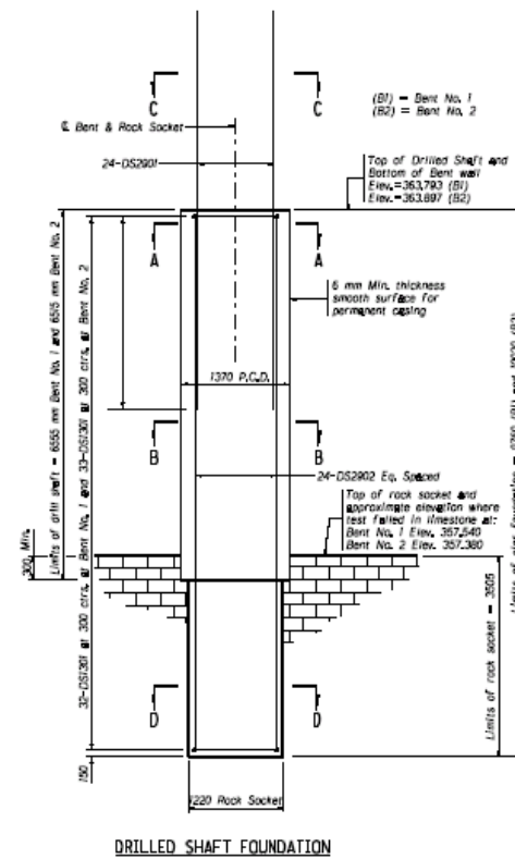
DRILLED SHAFT FOUNDATION
